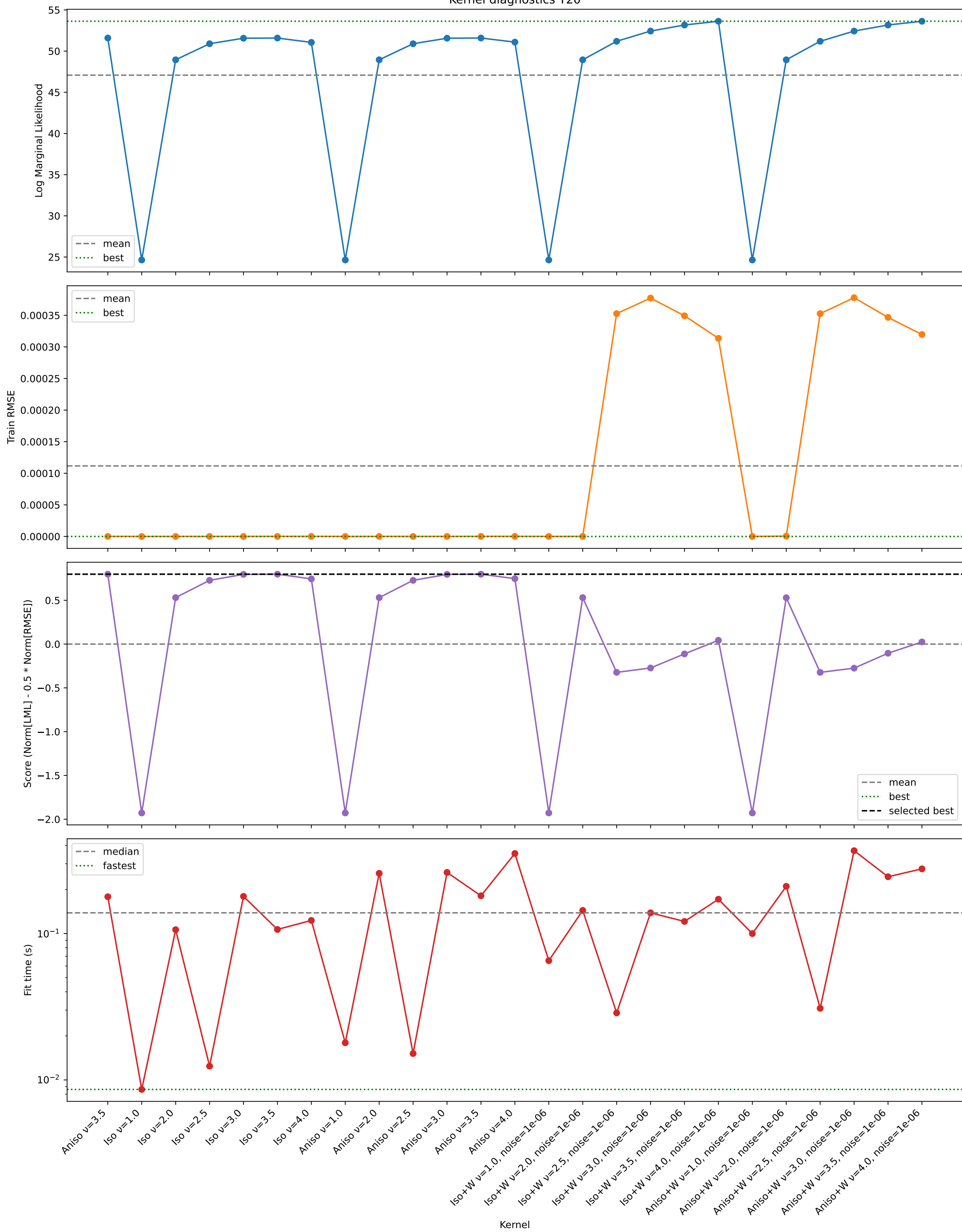
Kernel diagnostics T20
