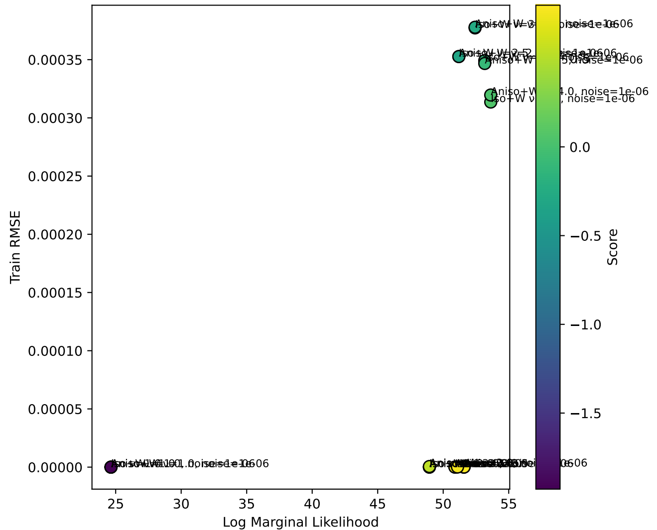
LML vs RMSE (T20)
