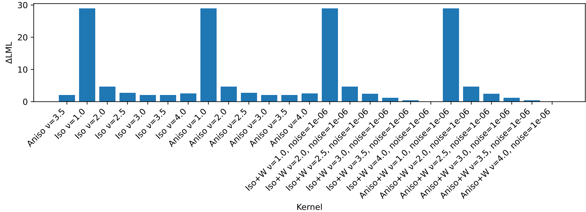
Difference from best LML (T20)
