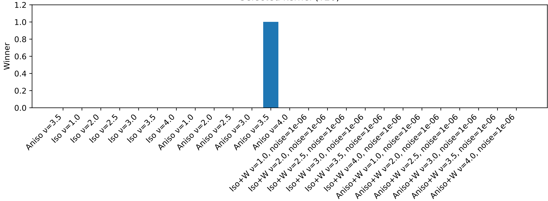
Selected kernel (T20)
